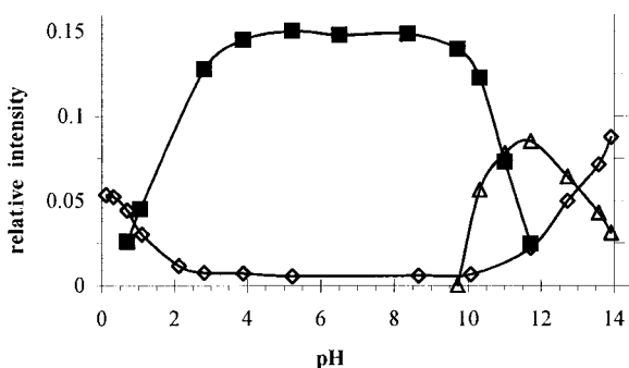
Fig. 2 The dependence of pH upon the normalised relative intensities of EPR signals obtained on TSA degradation by HO• at a flow rate of 125 ml h -1 : (◇) benzyl radical 1 , (■) hydroxycyclohexadienyl radical 5 , (△) phenoxyl radical (sum of radicals 2 and 3 ).
