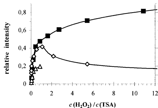
Fig. 3 The dependence of the molar ratio between H 2 O 2 and TSA (at a fixed TSA concentration of 70 mmol l -1 ) upon the normalised relative intensities (1/2 × ΔH pp × signal height) of EPR signals for TSA degradation by HO• radicals at a flow rate of 100 ml h -1 (◇) benzyl radical 1 at pH 0.6, (■) hydroxycyclohexadienyl radical 5 at pH 4.8, (△) phenoxyl radical at pH 12.6 (initial pH value).
