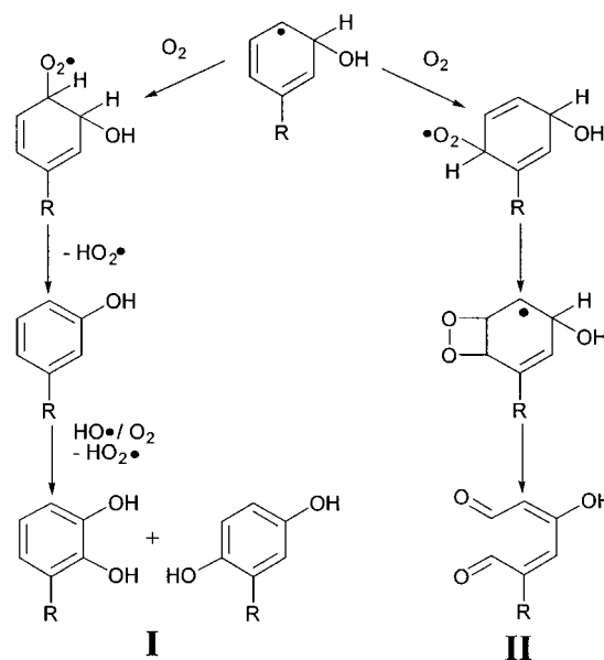
Fig. 7 Mechanism for consecutive reactions of hydroxycyclohexadienyl radicals with oxygen leading to different phenolic compounds and to bond breaking. 29,33,34,43,93
