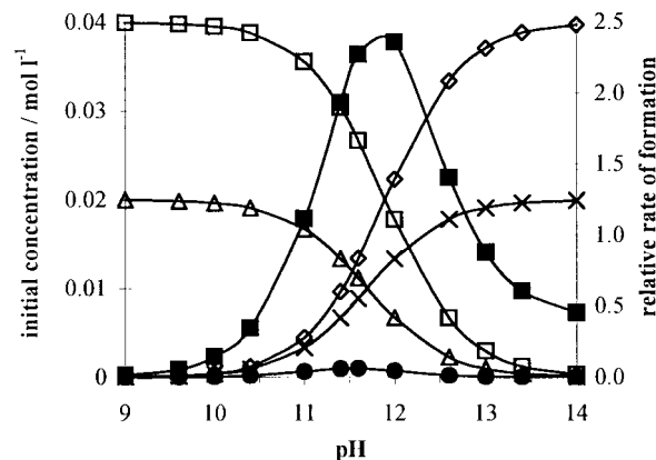
Fig. 9 Simulation of the relative rates of formation of the superoxide radical anion ( \blacksquare ) O_2\cdot^- and singlet oxygen ( \bullet ) ^1O_2 according to the rate constants (Table 3) dependence upon pH (assumed concentrations after photolysis: HO\cdot : 40 mmol l^{-1} , H_2O_2 : 20 mmol l^{-1} ). ( \diamond ) c(O_2\cdot^-) , ( \square ) c(HO\cdot) , ( \triangle ) c(H_2O_2) , ( \times ) c(HO_2^-) . Open symbols relate to the scale on the left, filled symbols to the scale on the right.
