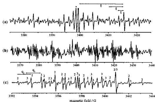
Fig. 1 The dependence of pH upon the EPR spectra obtained during TSA degradation by HO• radicals (q=quartet, t=triplet) (a) benzyl radical 1 and SO 3 • - (*) at pH 0.4 (25 ml h -1 ), (b) hydroxycyclohexadienyl radical 5 at pH 4.8 (90 ml h -1 ) (c) phenoxyl radicals 2 and 3 at pH 11.5 (20 ml h -1 ).
