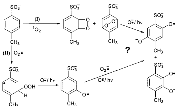
Fig. 8 Proposed mechanism for reactions of aromatic hydrocarbons with ^1O_2 and O_2\cdot^- leading to semiquinones. 29,94,95
