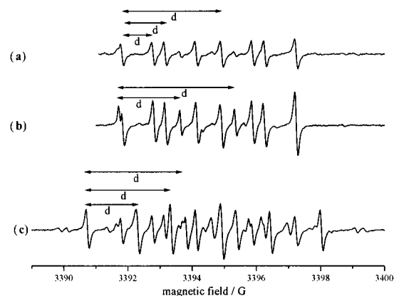
Fig. 5 The dependence of pH and flow rate upon the EPR spectra obtained during HSA degradation by HO• radicals (a) 17 at pH 11.5 (130 ml h -1 ), (b) 18 at pH 11.5 (10 ml h -1 ), (c) 21 at pH 13.5 (130 ml h -1 ).
